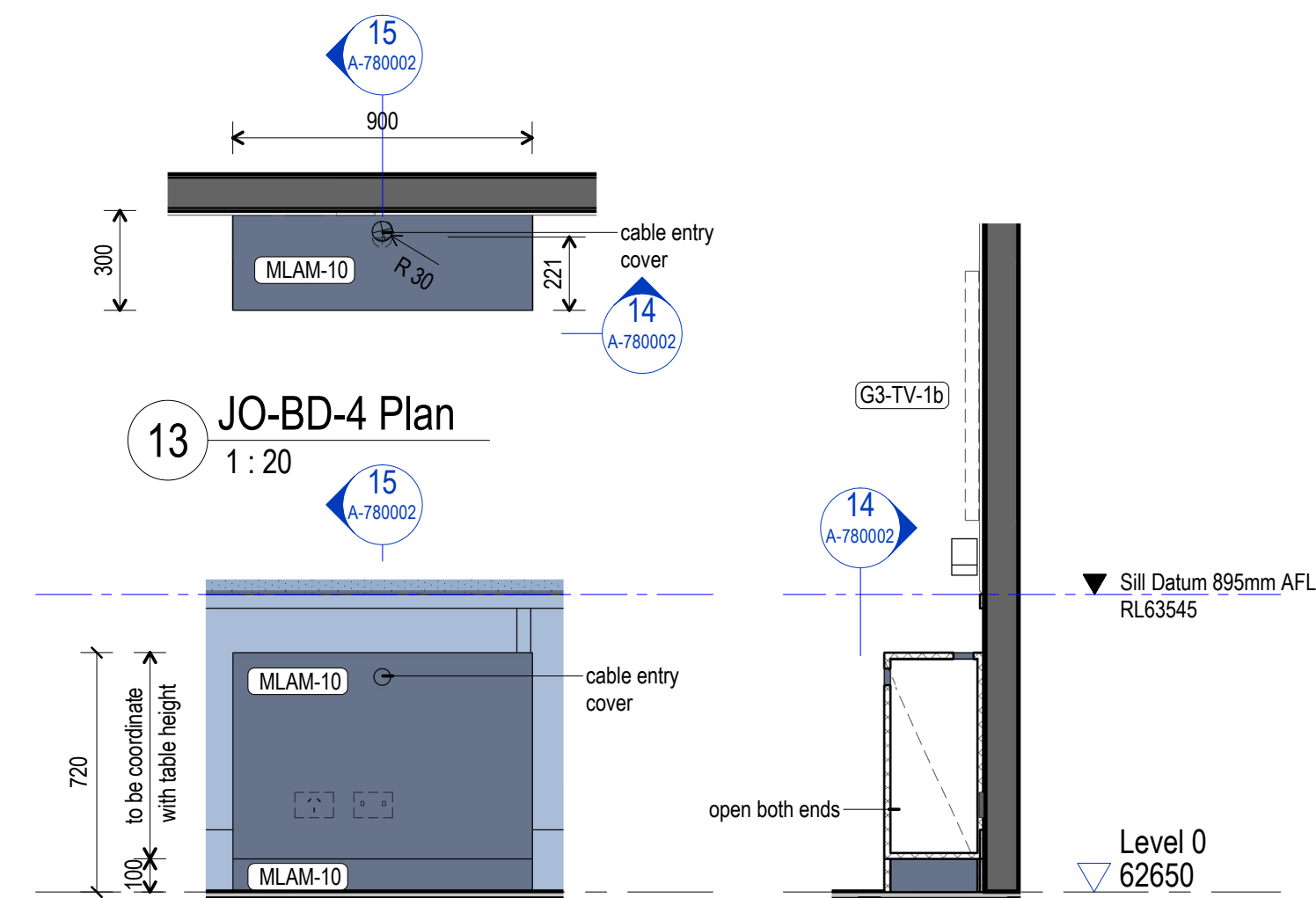
13 JO-BD-4 Plan 1:20
