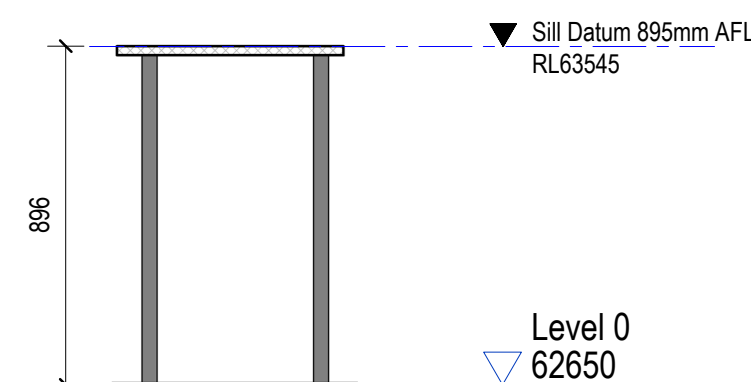
11 JO-BD-3 Section 1:20
